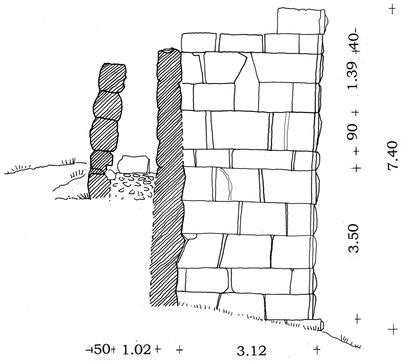
East façade / Cross section
